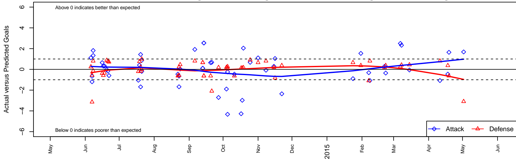
WPFC A pre-ECNL G01 Dots are actual minus expected GF (blue circles) and GA (red triangles). Blue line is smoothed change in attack strength. Red is smoothed change in defense strength.
